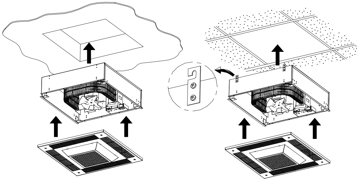
937 Series Recessed Mounting
